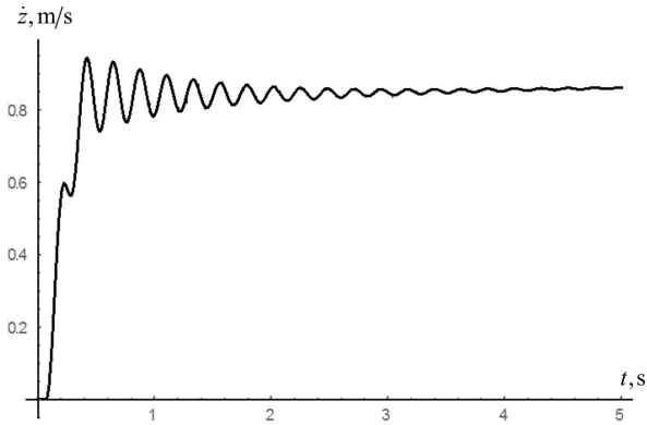
Fig. 3. Graph of the speed of the cart
